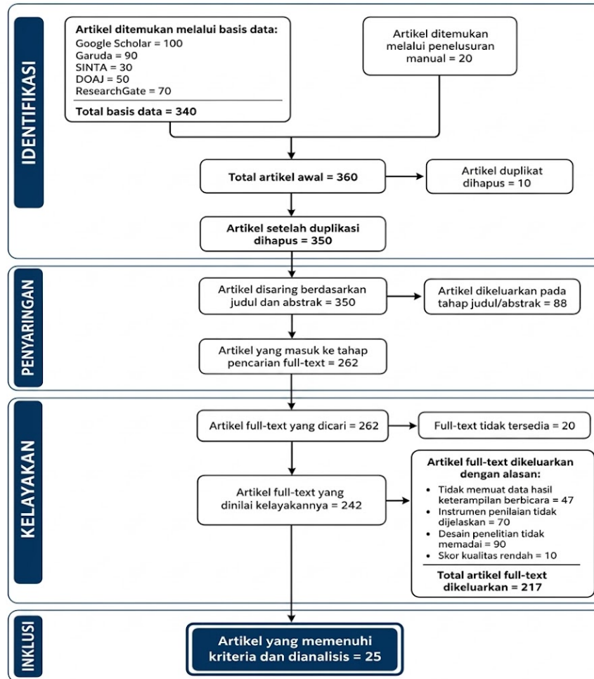
Gambar 1 Diagram PRISMA
